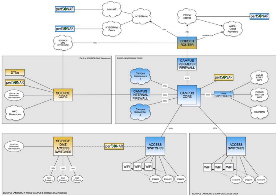
Items shown in blue are existing devices. Items in gold are proposed.
